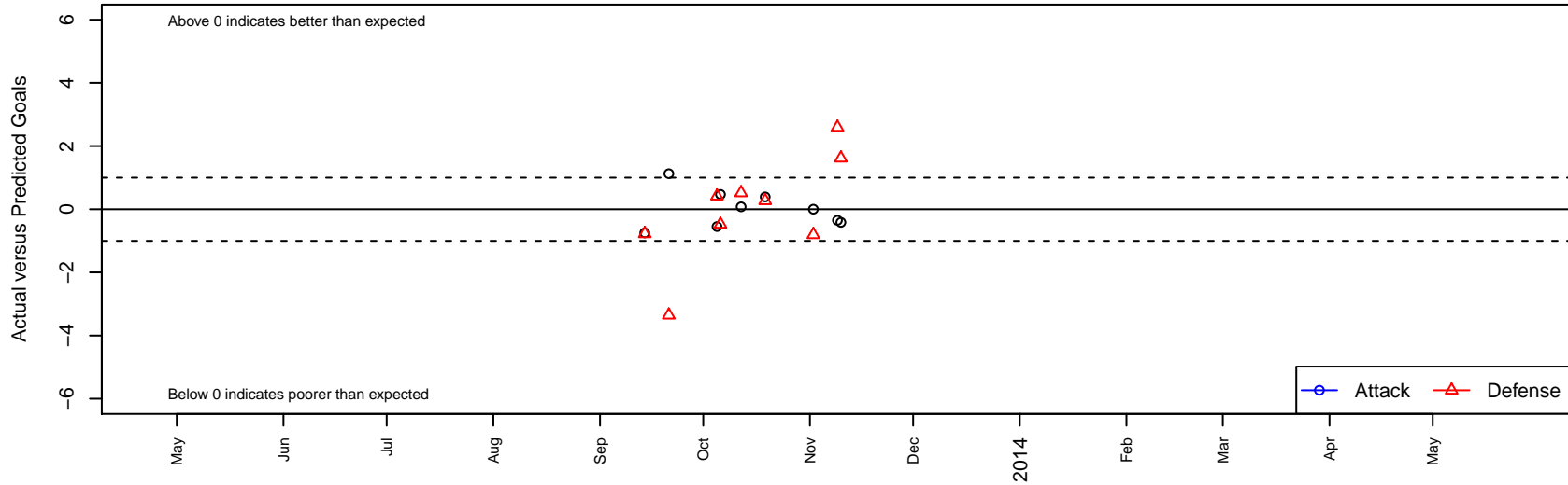
San Ramon 03 Azuri G02 Dots are actual minus expected GF (blue circles) and GA (red triangles). Blue line is smoothed change in attack strength. Red is smoothed change in defense strength.
